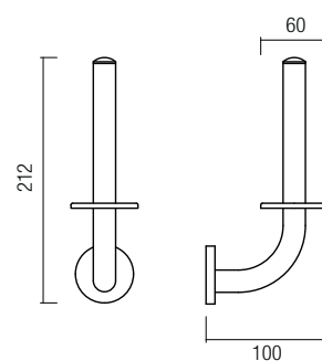
BA 721 - Spare Paper Holder
