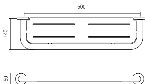
BA 708 - 500 mm Stainless Steel Shelf
