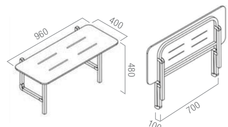
SS 964 SS 960 mm x 400 mm Max Load: 160 kg (25 Stone) White Seat/Stainless Steel Frame AS 1428.1-2009 Compliant
