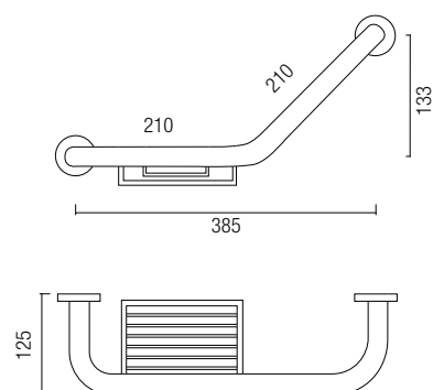
CR 036 - Ramped Comfort Rail with Soap Basket Suitable for either left or right hand installation.
